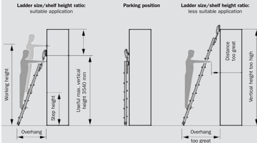
FRS shelf ladder with guide rail (inclined) – for example R 4000
