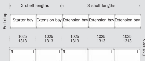
The positioning of the left and right brackets within the rows of shelving (top view)
