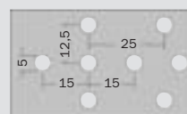
Euro hole sizes, dimensions in mm
